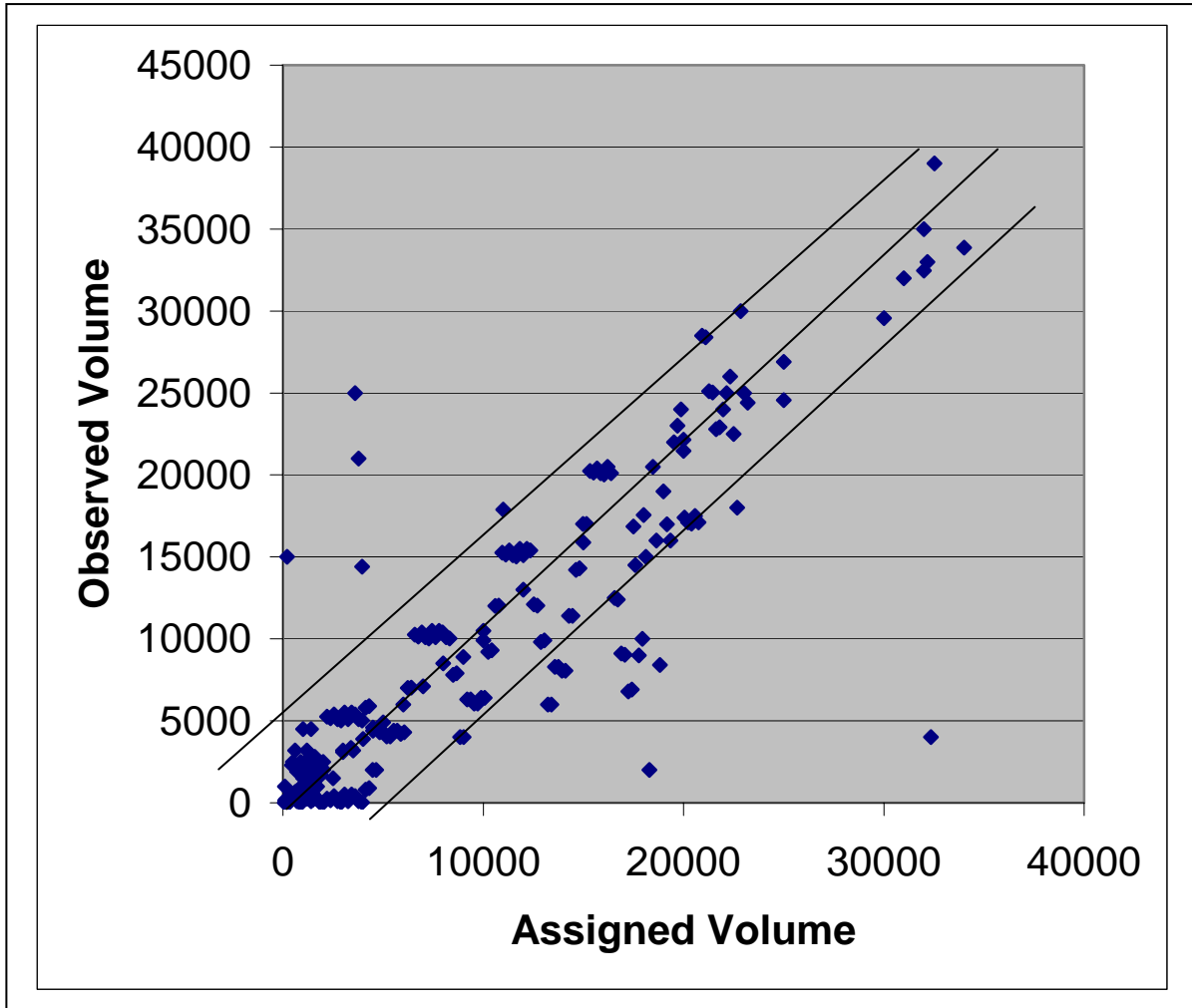
Figure 3- Scatter Plot of Assigned vs. Observed Link Traffic Volume
