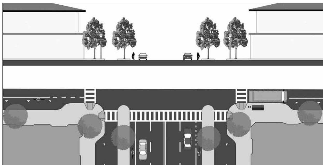
Figure 6.6 A multiway boulevard is characterized by a central roadway with a pair of one-way access lanes. This type of thoroughfare can combine high vehicular capacity with pedestrian-friendly streetsides. Source: Digital Media Productions.
